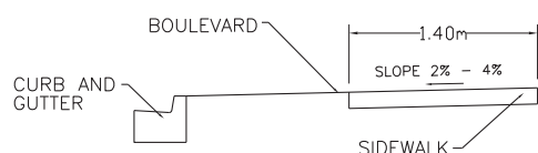
Figure 4.1.10.7A Concrete Sidewalk With Boulevard
