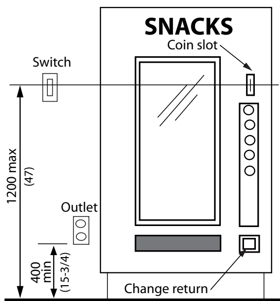
Figure 4.4.3.1 Vending Machine
