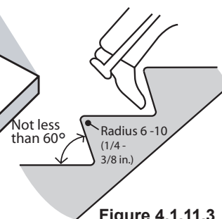
Figure 4.1.11.3 Raked Riser
