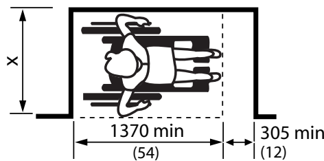
Figure 4.1.1.4 Clearances at Alcove
