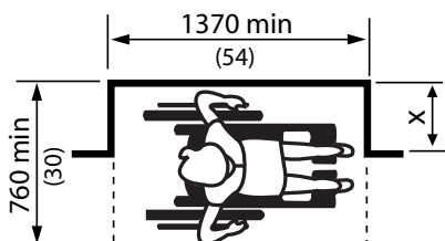
Figure 4.1.1.2 180° Turning Space
