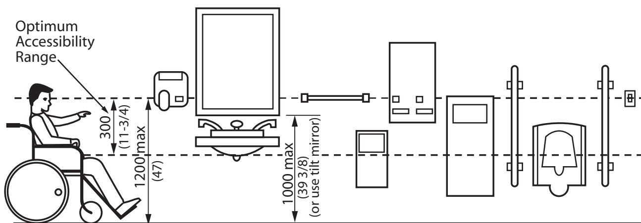
Figure 4.2.6.1 Washroom Accessories
