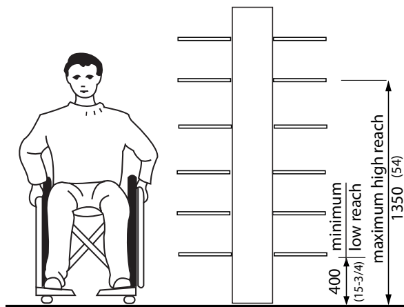
Figure 4.5.6.2 Reach Heights
