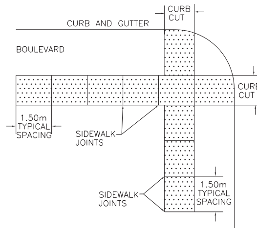
Figure 4.1.10.7C Layout of Sidewalk Joints
