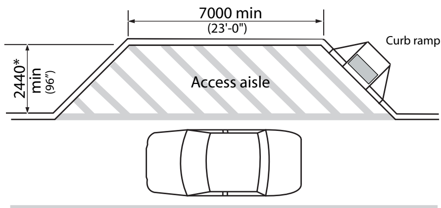
Figure 4.3.13.2 Passenger Loading Zone (Dimensions in mm)
