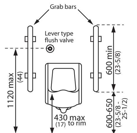
Figure 4.2.5.2 Urinal
