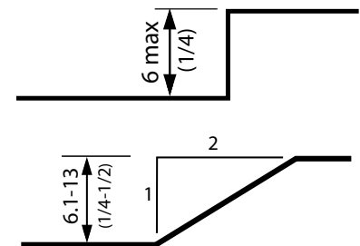
Figure 4.1.2.1 Changes in Level
