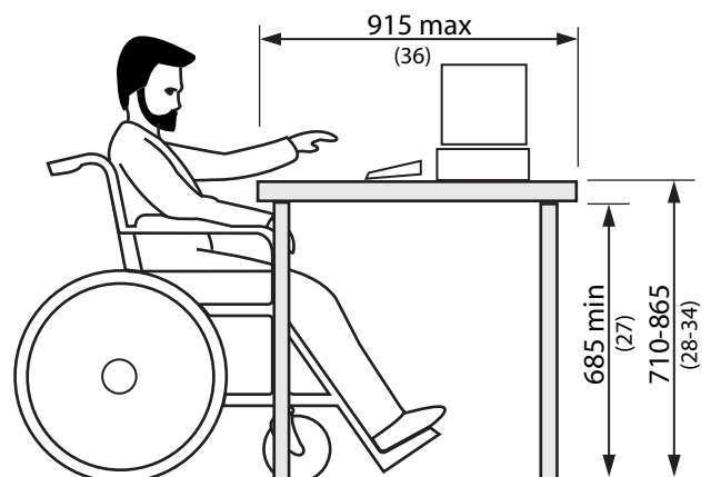
Figure 4.5.6.3 Work Surfaces
