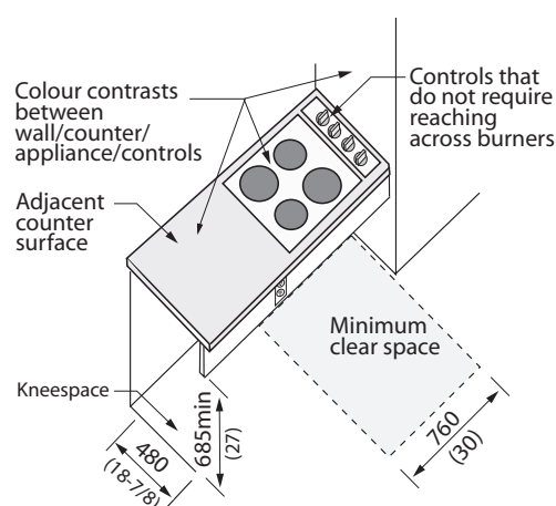
Figure 4.3.18.6 Cook Top
