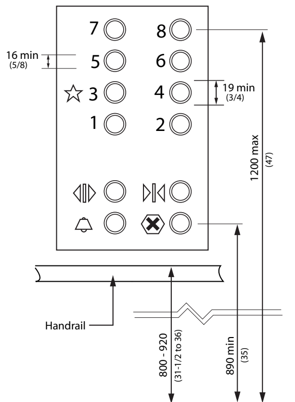
Figure 4.1.14.2 Control Panel
