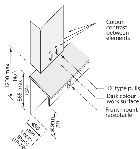
Figure 4.3.18.4 Storage Elements
