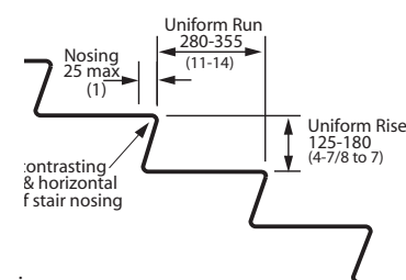
Figure 4.1.11.2 Stair Tread Criteria
