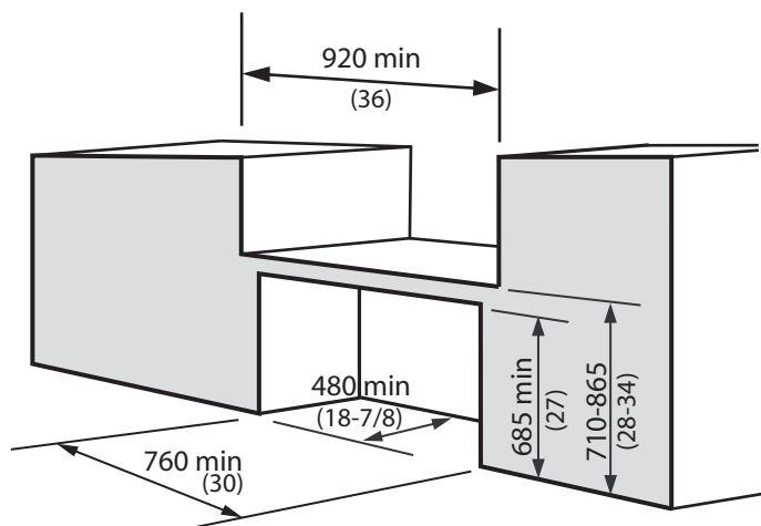
Figure 4.3.8.1 Service Counter
