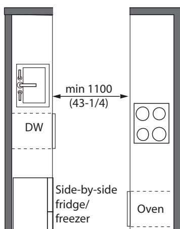
Figure 4.3.18.1 Pass-Through Kitchen
