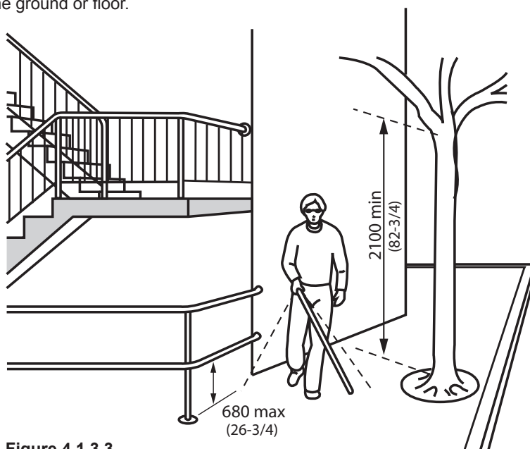
Figure 4.1.3.3 Overhead Obstructions
